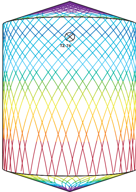
D5m H6m, Toftejorg TZ-74 Self Cleaning version, 4 x ø7 mm, 0% Time = 3.8 min., Water consumption = 1192 l (315 gallon)
